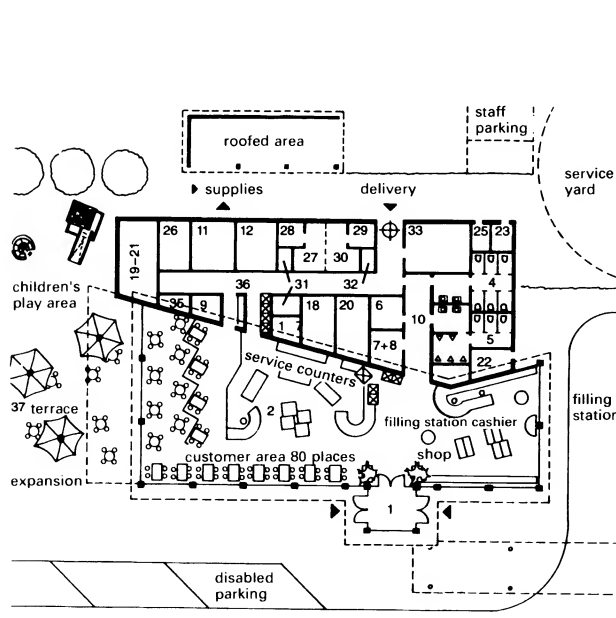
② Petrol and service station for 80 people
